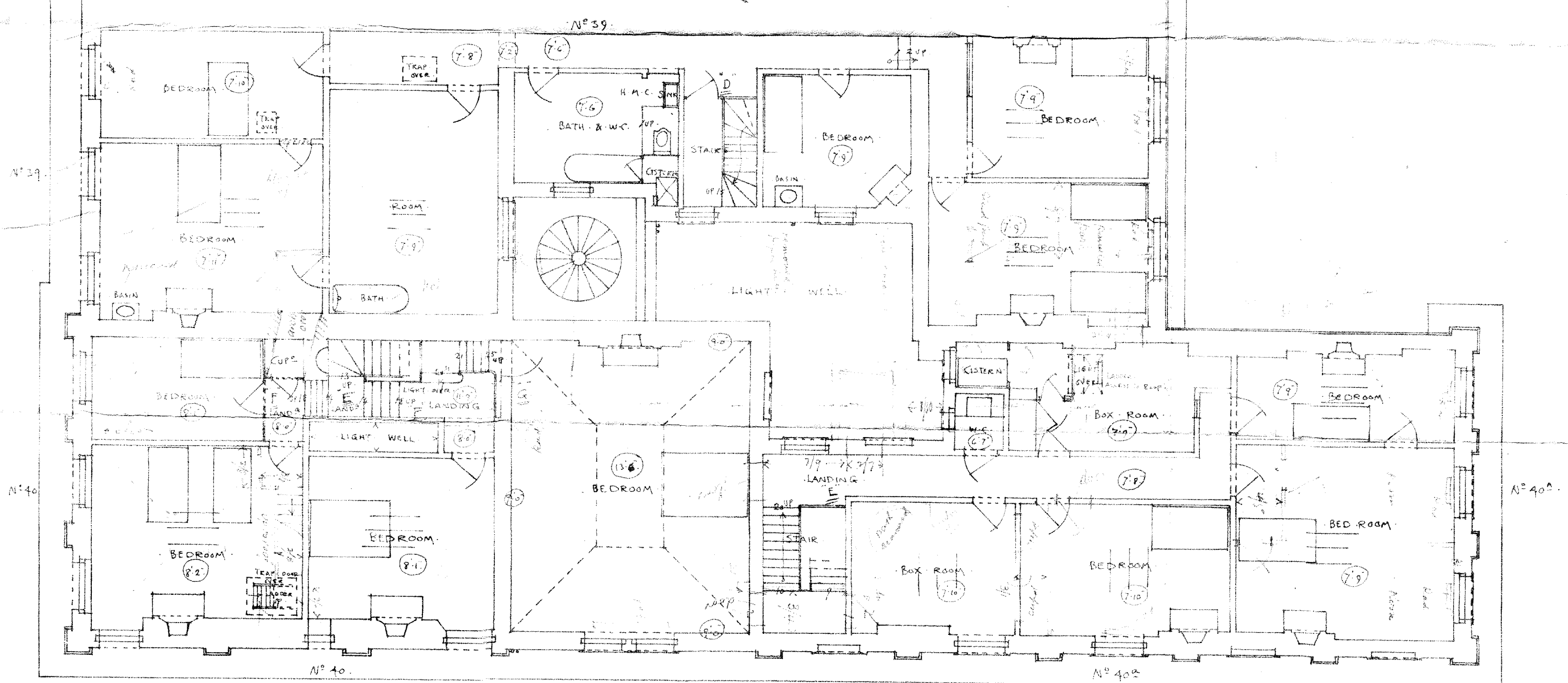
PLAN OF THIRD FLOOR LEVEL.
