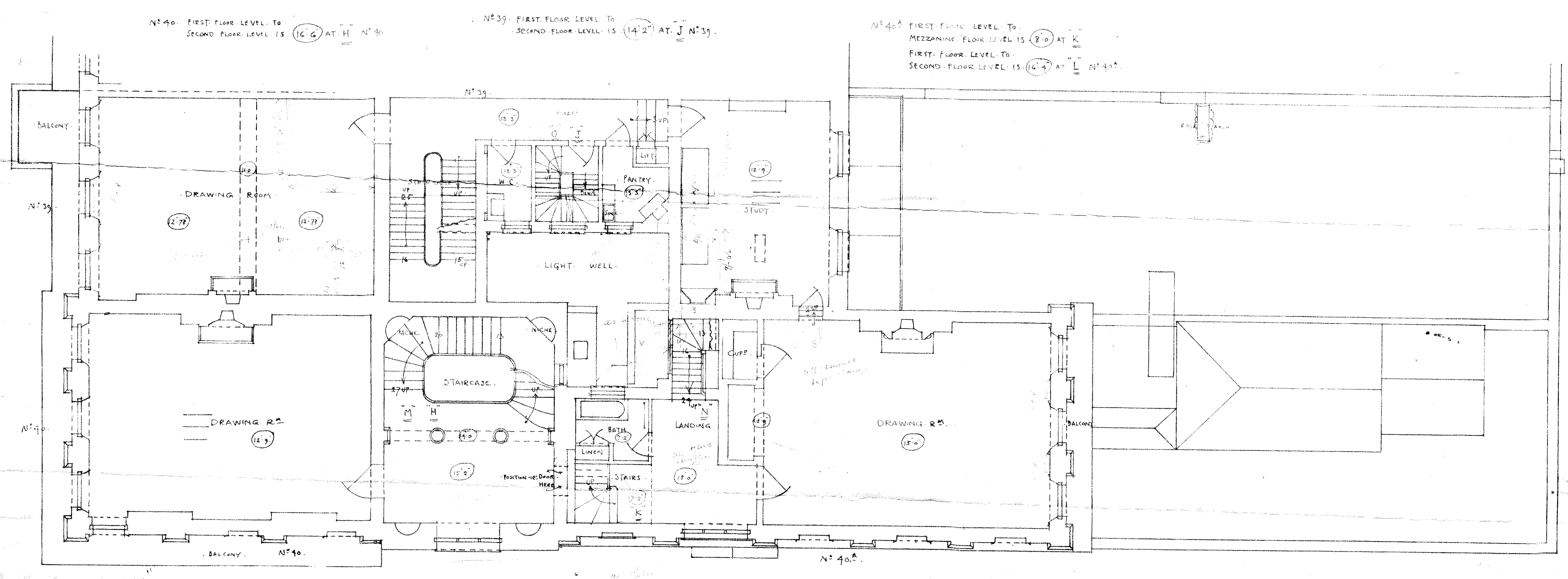
PLAN OF FIRST FLOOR LEVEL.
